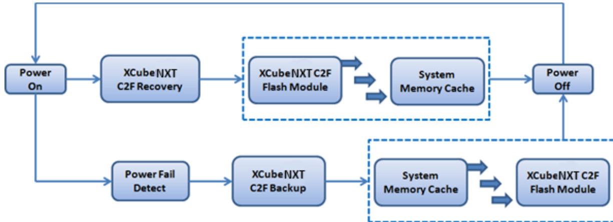
Figure 2-14 Cache-to-Flash Workflow
